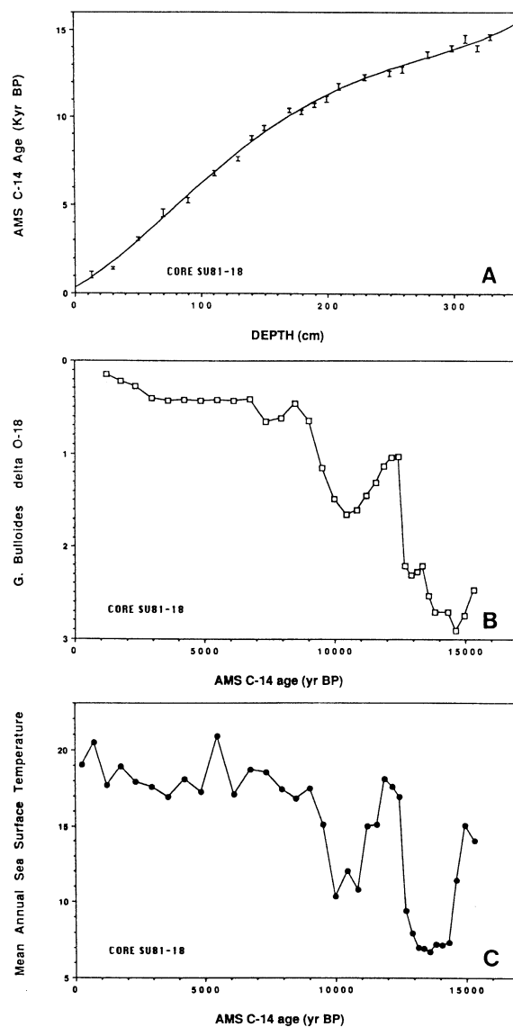
Fig 1. A. Sedimentation rate of core SU81-18; B. Variations of the oxygen isotope ratio of the planktonic foraminifer G. bulloides vs ^{14}C age in core SU81-18; C. Variations of the sea surface temperature estimate vs ^{14}C age in core SU81-18
