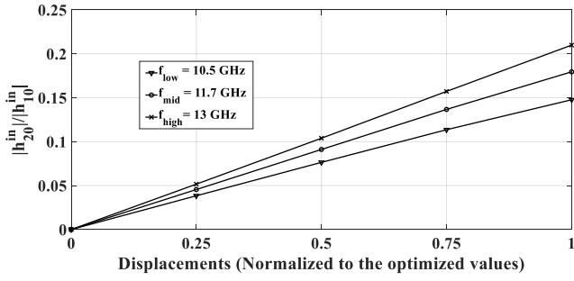
Fig. 3. Parametric analysis for the progressive excitation of the modal amplitude ratio |h_{20}^{in}|/|h_{10}^{in}| on the output of each of the four excitation waveguide parts.
