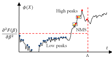
Figure 2: Key-frame selection
