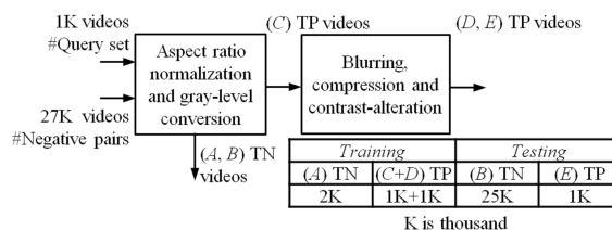
Figure 3: Pipeline to process the SVD dataset K is thousand
