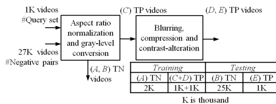
Figure 3: Pipeline to process the SVD dataset K is thousand
