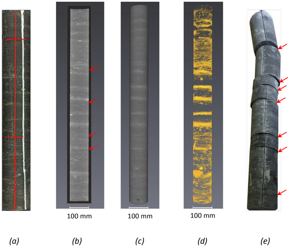
891 Figure 1. Photos and CT scans of core 5: a) Photo at initial state; b) to d) CT scan prior to sending to lab; e) Opening 892 in lab. 893 894
