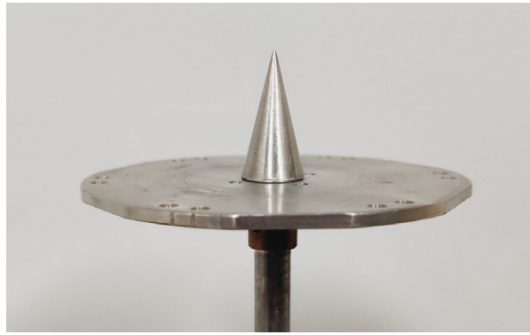
Figure 4. The shape of the SEIS foot. The conical spike has a maximum diameter of 10 mm.
