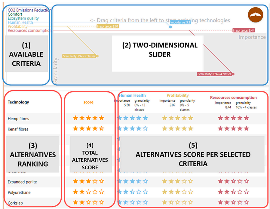
Fig. 5. Proposed UI.
