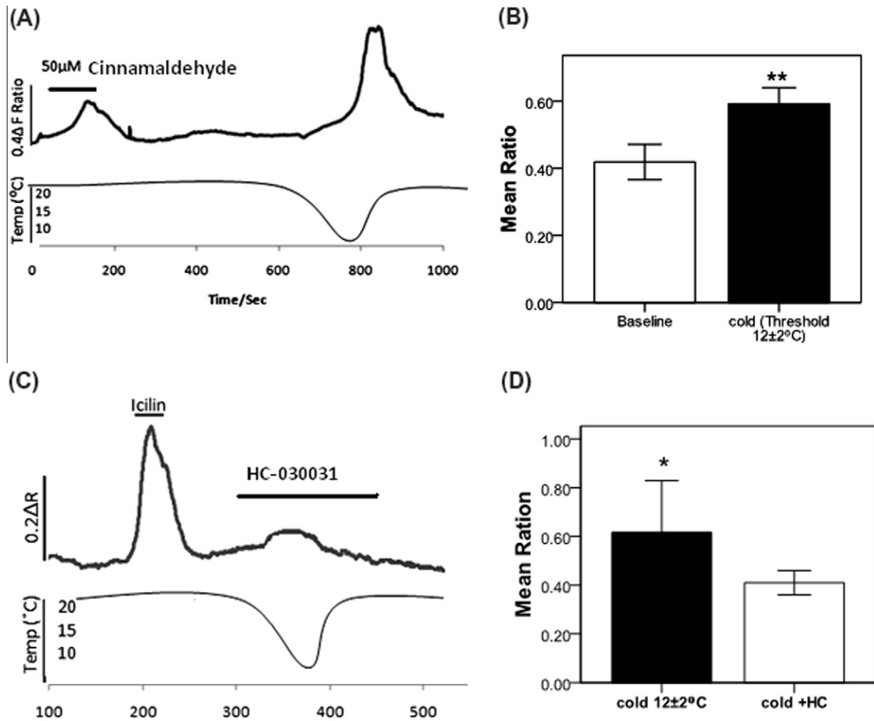
Fig. 7. Responses of odontoblast-like cells to noxious cold stimulation. (A) Cinnamaldehyde responsive cell showed response to cold stimulus, (threshold 12 \pm 2^{\circ}C ) and (B), bar chart summary of cell responses to noxious cold stimuli ( n = 23 ). Cell responses to cold were attenuated pharmacologically with TRPA1 antagonist M HC-030031 (C and D) and with gene suppression of TRPA1. (E) Western blot analysis of TRPA1 protein following 72 h cells transfection with TRPA1 siRNA and control scrambled siRNA. Protein expression decreases in a concentration dependent manner with significant knockdown at 50 nM compared to control. (F) TRPA1 siRNA transfected cell (ii) showing no response to cinnamaldehyde or cold (threshold 12 \pm 2^{\circ}C ), while a control cell (i) showed response to both. (G) Bar chart of average responses of control and TRPA1 siRNA transfected cells to cold ( n = 12 ) (threshold 12 \pm 2^{\circ}C ), error bars indicate SEM, paired Student t test ** p \leq 0.01 , * p \leq 0.05 .
