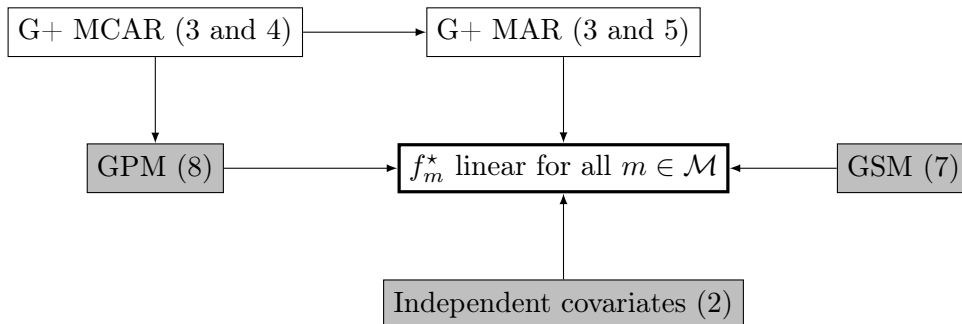
Figure 2: Links between the different assumptions to get the linearity of the Bayes rule as in Proposition 2.7. Scenarios that may contain MNAR cases are depicted in gray.
