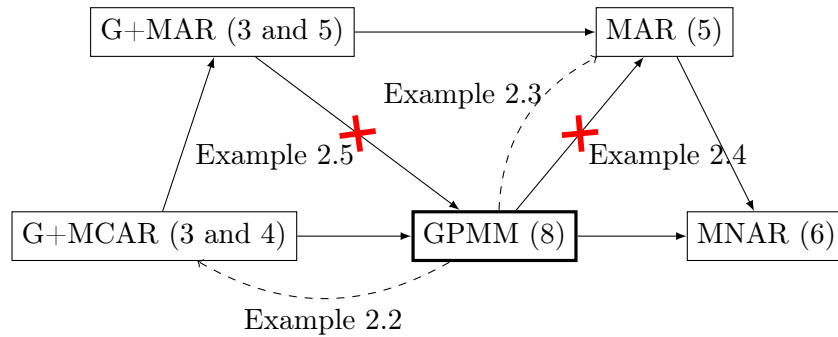
Figure 1: Links between Gaussian pattern mixture models (GPMM) and Gaussian selection models. Solid arrows correspond to inclusions, dotted (resp. crossed) arrows illustrate a partial inclusion (resp. non-inclusion).
