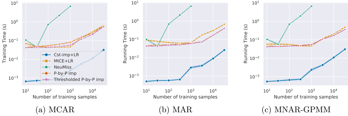
Figure 5: Training time w.r.t. the number of training samples.
