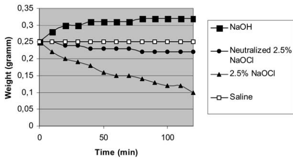
Fig. 1. Weight variation over 120 minutes of palatal mucosa samples placed in 2.5% NaOCl, neutralized 2.5% NaOCl, NaOH, and saline. The Kruskal and Wallis test showed a statistically significant difference among the 4 liquids. The samples stored in NaOH gained weight, those placed in saline did not vary, and those soaked in 2.5% NaOCl lost more weight than in neutralized 2.5% NaOCl.
