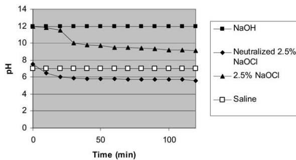
Fig. 2. pH variations over 120 minutes of solutions containing pig palatal mucosa samples. The pH of saline and NaOH did not vary but that of the 2.5% NaOCl and neutralized 2.5% NaOCl solutions decreased respectively from 12 to 9 and from 7.5 to 5.6.
