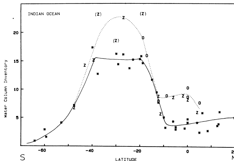
Fig 3A. Plots of water column bomb ^{14}\text{C} inventories, expressed in 10^9 atoms/cm ^2 , as a function of latitude
