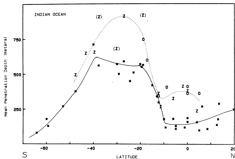
Fig 3B. Plots of mean penetration depth as a function of latitude. For conventions see Fig 3A.
