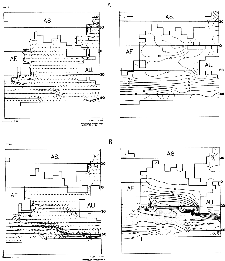
Fig 6. \Delta^{14}\text{C} for the year 1990 (right) and horizontal velocities (left) calculated with the GFDL model. (Fig 6A: level 2, 85m; Fig 6B: level 6, 755m). Heavily shaded areas indicate maxima \Delta^{14}\text{C} > -40\text{‰} ; lightly shaded areas indicate minima ( \Delta^{14}\text{C} < 0\text{‰} for 6A and < -120\text{‰} for 6B). The arrowheads are proportional to the horizontal velocities and appear when the magnitude is > 1.342\text{cm/sec} for level 2 and > 0.4472\text{cm/sec} for level 6. The brackets at lower left and lower right beyond the frames scale the arrowshafts in cm/sec. The vector arrows for level 6 have been scaled up by a factor 3 over the scaling used for level 2.
