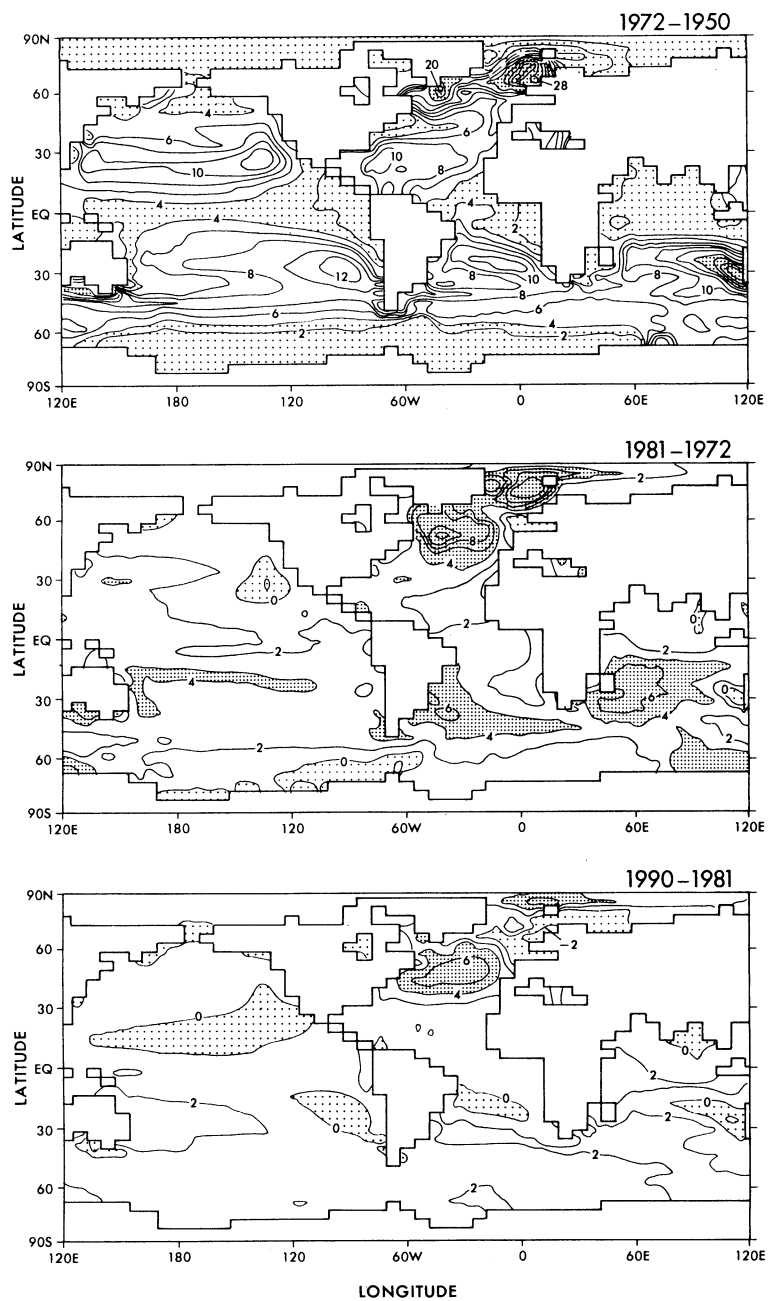
Fig 4. Water-column inventories of bomb ^{14}\text{C} calculated with the GFDL model. 4A: 1972; 4B: 1981 minus 1972, 4C: 1990 minus 1981. Heavily shaded areas indicate maxima (for 4A: > 16.10^9 atoms/cm ^2 , for 4B and 4C: > 4.10^9 atoms/cm ^2 ); lightly shaded areas indicate minima (for 4A: < 4.10^9 atoms/cm ^2 , for 4B and 4C: < 0 ).
