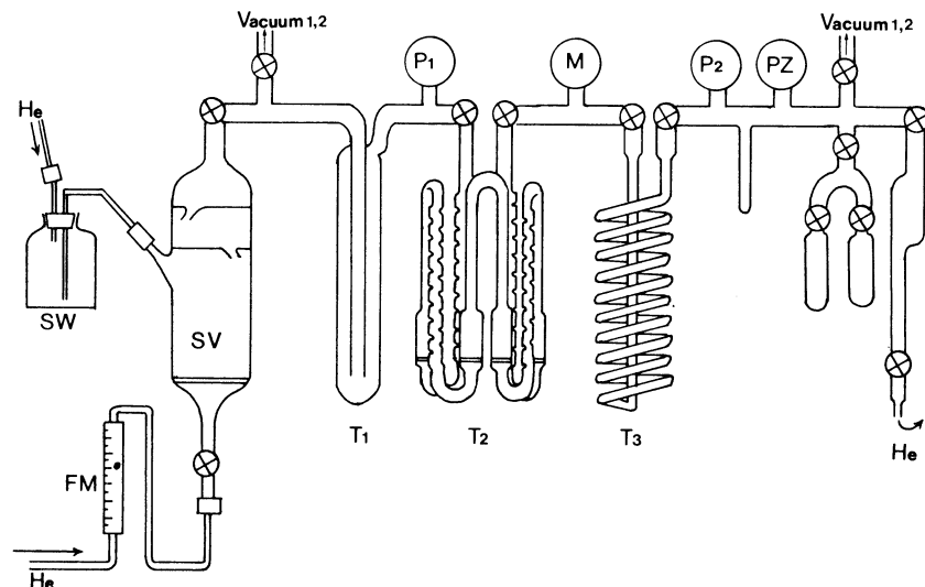
Fig 1. Schematic description of the \text{CO}_2 extraction system (CFR). T_1 , T_2 , T_3 = cold traps (respectively at -75^\circ\text{C} , -75^\circ\text{C} and -190^\circ\text{C} ); P_1 , P_2 = Pirani gauges; M = manometer; PZ = piezoresistive pressure gauge; vacuum 1, 2 = vacuum generated by a primary rotary pump and an oil diffusion pump; SV = stripping vessel; FM = flow-meter, SW = seawater sample
