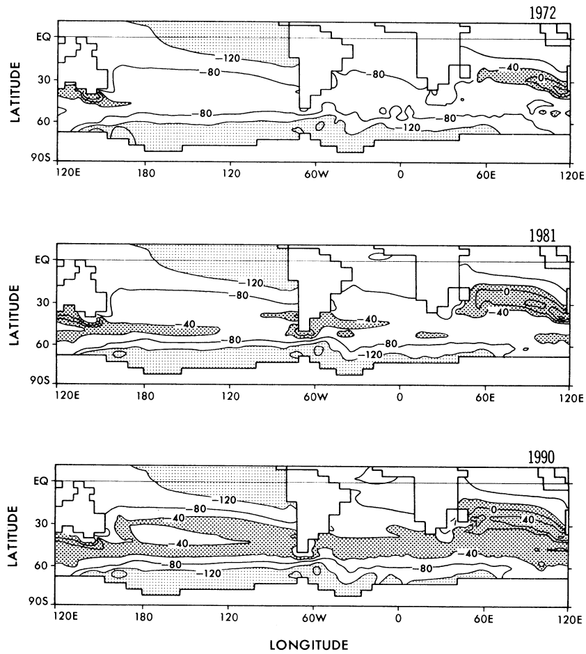
Fig 5. \Delta^{14}\text{C} calculated with the GFDL model at intermediate depth (level 6: 755m). (5A: 1972; 5B: 1981; 5C: 1990). Heavily shaded areas indicate maxima ( \Delta^{14}\text{C} > -40\text{‰} ); lightly shaded areas indicate minima ( \Delta^{14}\text{C} < -120\text{‰} ).
