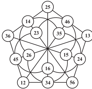
Figure 7: A duad-syntheme model of W(3,2) .
