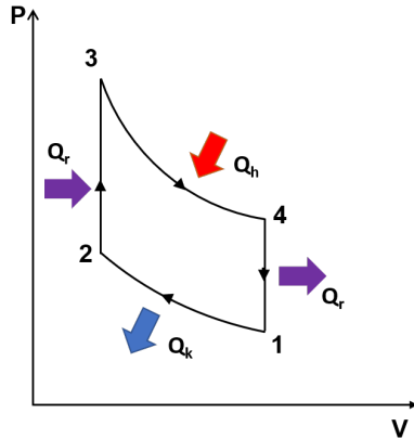
Figure 1 : Cycle de Stirling
