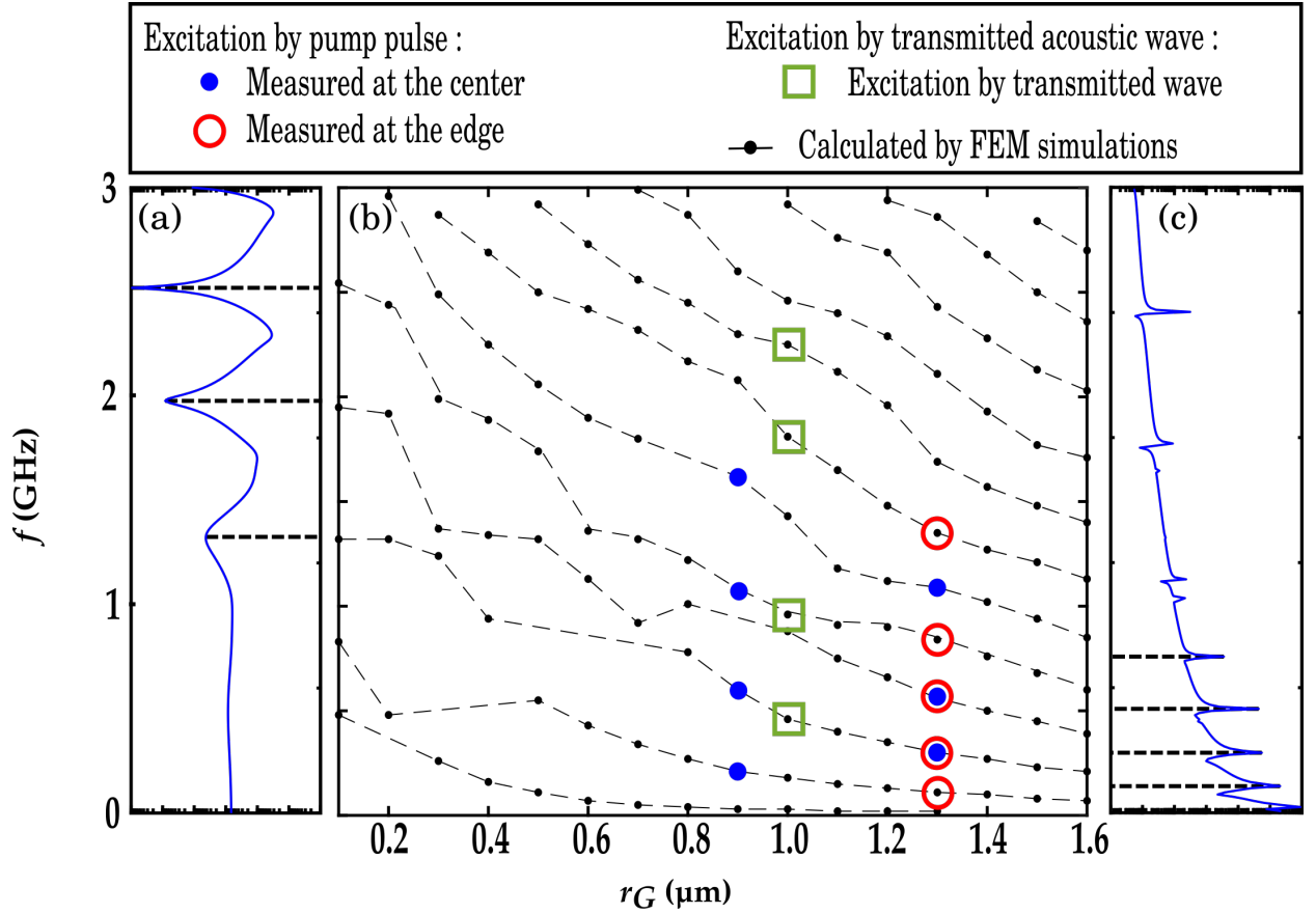
FIG. 7. (a) Spectrum obtained by a simulation for a disk in contact with silicon substrate. (b) Frequency obtained by simulations and identified as modes for different values of r_G . Experimental values are also reported for comparison. (c) Spectrum obtained by a simulation for a free disk without silicon substrate
