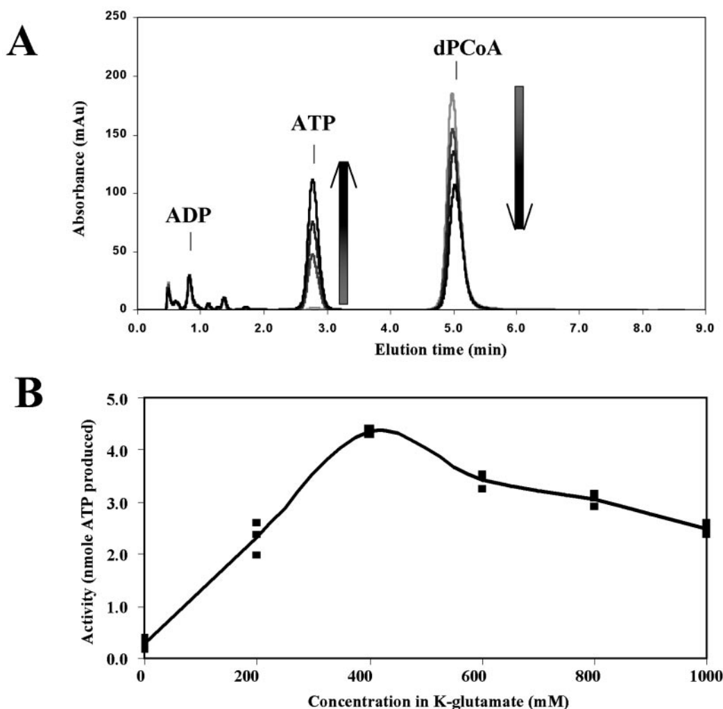
FIG. 4. Reverse PPAT activity assay. A , synthesis of 4'-phosphopantetheine and ATP from PP i and dPCoA analyzed using an HPLC-based assay. Samples were incubated for 0 ( light line ), 1 ( medium line ), 2 ( dark line ), and 4 ( darkest line ) min in the presence of PAB0944, diluted in fresh dithiothreitol solution, and subjected to isocratic separation on a Supelcosil LC-18 reverse-phase column. Pure dPCoA, ATP, ADP, and phosphopantetheine solutions resolved in similar conditions were used as standards. Absorbance at 255 nm was used to follow the elution of these compounds. Arrows indicate the evolution over time of the concentration of the two detectable compounds. B , influence of potassium glutamate on reverse PPAT activity. The reverse PPAT reaction was carried out in 50 mM Tris/HCl buffer (pH 8.0) containing 0–1000 mM potassium glutamate. PAB0944 (88 nM) was incubated at 85 °C with 0.25 mM dPCoA, 2 mM inorganic phosphate, 2 mM MgCl 2 . The total activity after 4 min from 40 μl of the reaction was estimated in triplicate assays by HPLC measurements.
