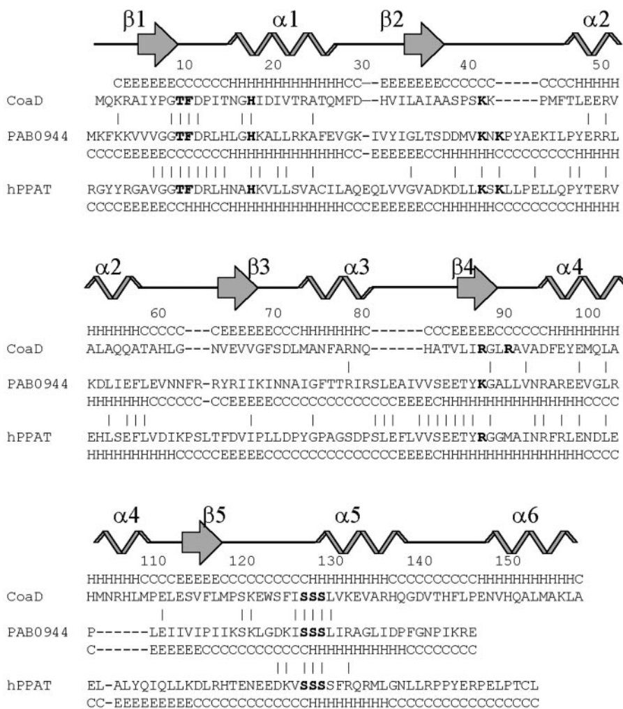
FIG. 7. Sequence comparison between PAB0944 from P. abyssi , CoaD from E. coli , and the human PPAT domain. Prediction of secondary structure elements of PAB0944 were made through the Pspired web-interfaced software (Footnote 4) with the 1b6t structure of CoaD from E. coli as model. The alignment between the three polypeptides was manually corrected. Numbering is indicated for the CoaD sequence from E. coli . Important residues cited under "Discussion" are indicated in boldface . \beta -Sheets ( E ) are represented by arrows and \alpha -helices ( H ) are numbered based on the CoaD structure. Identical residues between PAB0944 and CoaD (14%) as well as between PAB0944 and the human PPAT domain (32%) are indicated by I .
