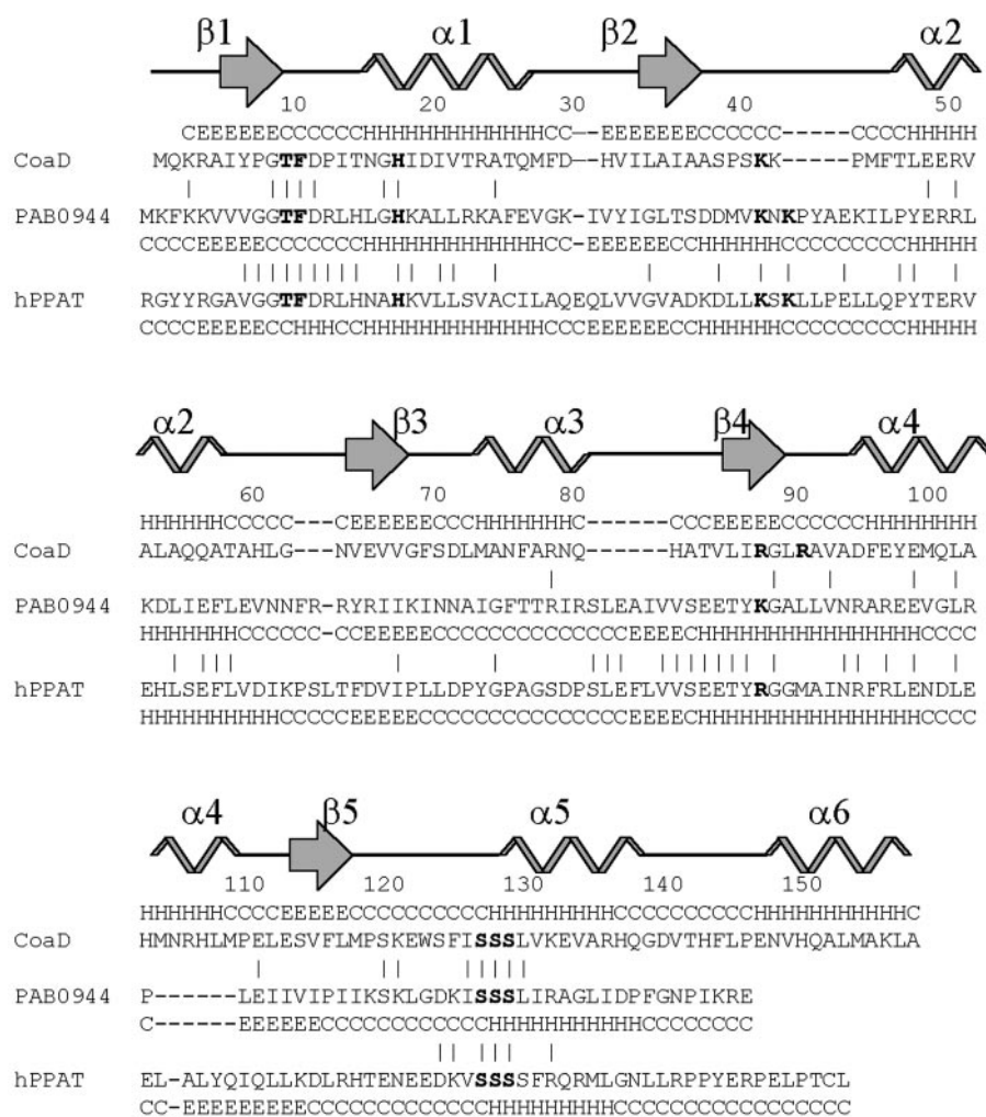
FIG. 7. Sequence comparison between PAB0944 from P. abyssi , CoaD from E. coli , and the human PPAT domain. Prediction of secondary structure elements of PAB0944 were made through the Pspired web-interfaced software (Footnote 4) with the 1b6t structure of CoaD from E. coli as model. The alignment between the three polypeptides was manually corrected. Numbering is indicated for the CoaD sequence from E. coli . Important residues cited under "Discussion" are indicated in boldface. \beta -Sheets ( E ) are represented by arrows and \alpha -helices ( H ) are numbered based on the CoaD structure. Identical residues between PAB0944 and CoaD (14%) as well as between PAB0944 and the human PPAT domain (32%) are indicated by I .
