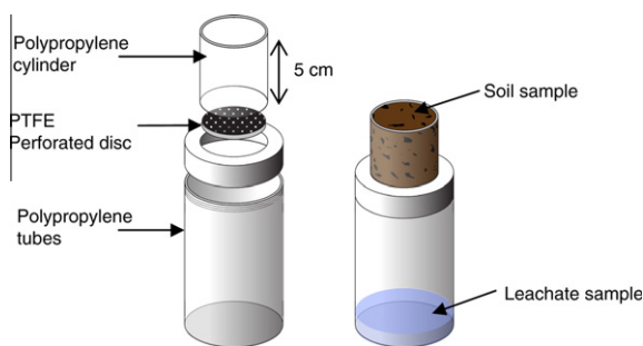
Fig. 1. Soil column devices with an exploded diagram.
