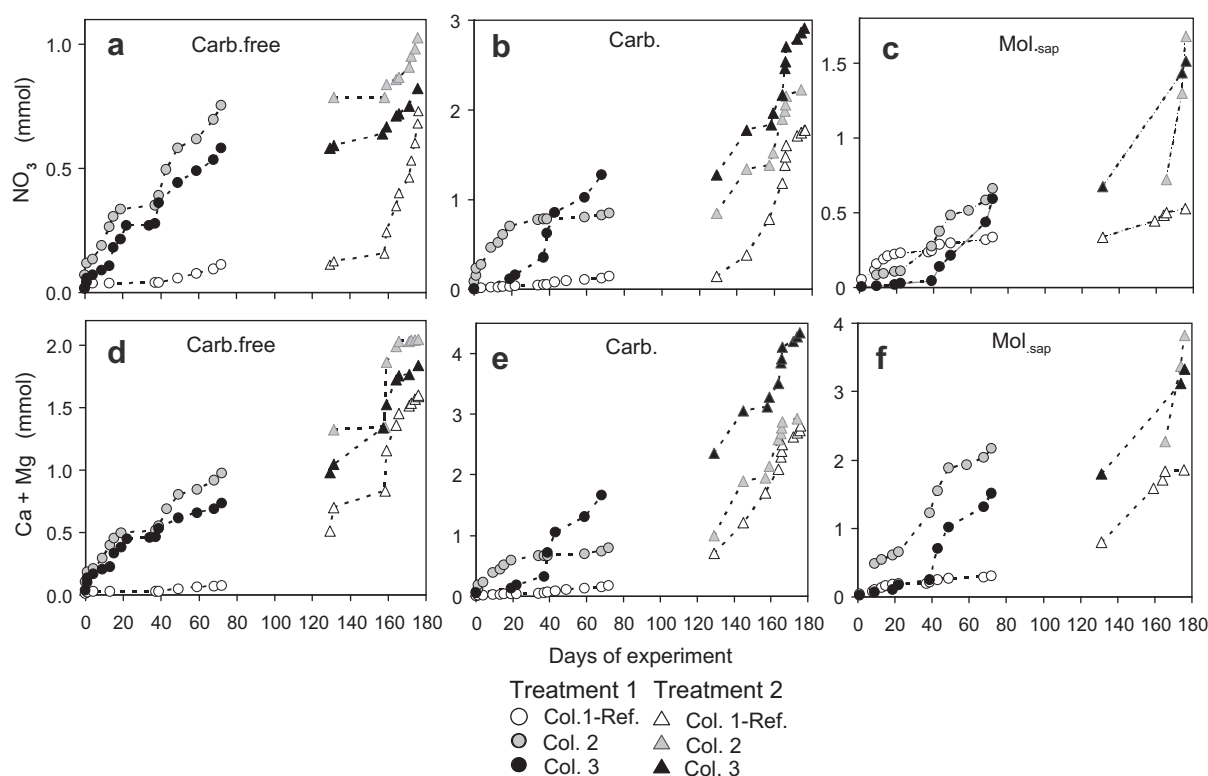
Fig. 3. Cumulative (Ca + Mg) and \text{NO}_3 fluxes (in mmol) in the leachates of carbonate free, carbonate and molasse saprolite soil columns over the time of experiment. The first experiment last from day 0 to day 72 and the second experiment from day 129 to day 176. (a) and (d): carbonate free soil; (b) and (e): carbonated soil; (c) and (f): molasse soil.
