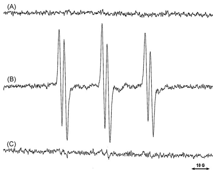
Fig. 2. In vitro detection of radical adducts. (A) Free radical generation in presence of DWCNTs: electron paramagnetic resonance spectra of N-tert-butyl-a-(4-pyridyl)-nitron N'oxide (4-POBN) radical adducts following the incubation with DWCNTs. (B) Positive control: ESR spectrum of POBN/ \bullet OH adduct detected after Fenton reaction as control. (C) same as B with addition of DWCNTs.
