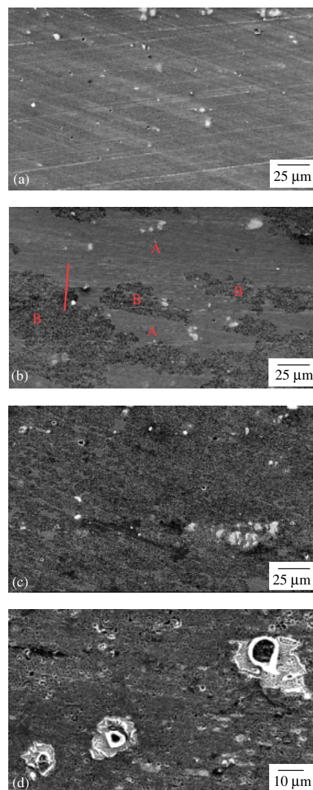
Figure 5. Scanning electron micrographs of an AA7075 T6 aluminium alloy that had been mechanically polished to 1 \mu m diamond paste finish and anodically polarised to various potentials indicated in Fig. 4, revealing surface appearance changes after anodic polarisation: (a) potential A; (b) potential B; potential C; (d) potential D.
