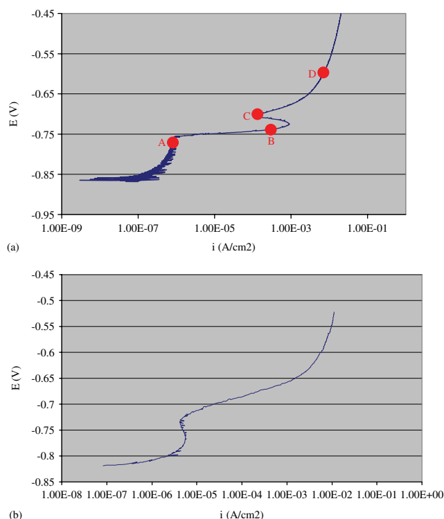
Figure 4. Anodic polarisation curves of AA7075 T6 aluminium alloy in 0.5 M NaCl solution: (a) mechanically polished to 1 \mu m diamond paste finish; (b) etched in 10 wt% NaOH solution.
