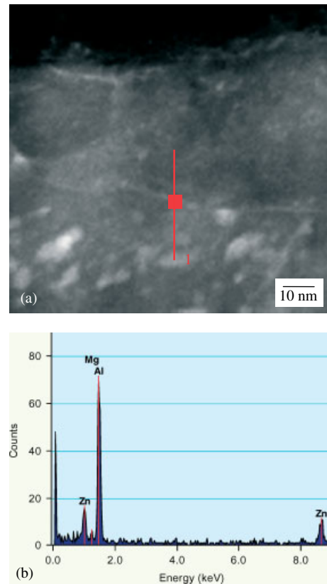
Figure 2. (a) High angle annular dark-field image of the framed area in Fig. 1; (b) EDX spectrum obtained at a grain boundary.
