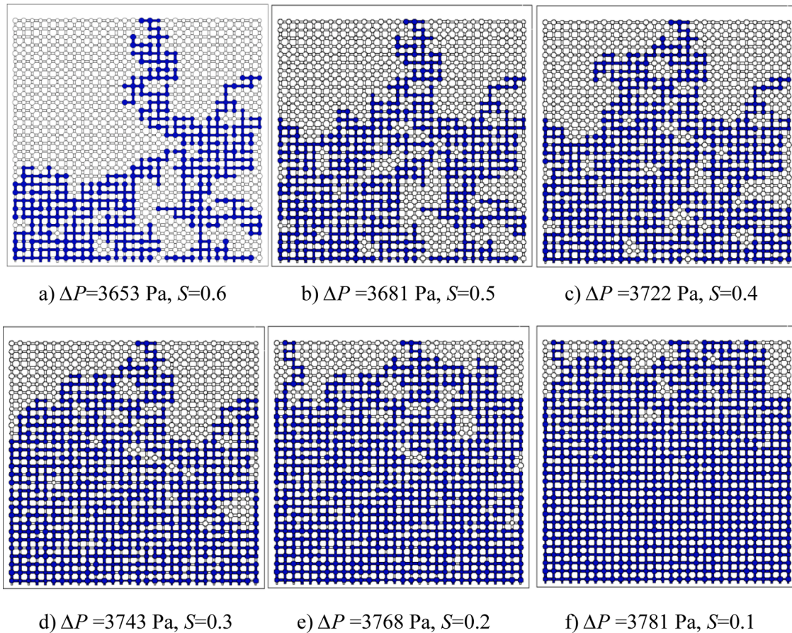
Fig. 2. Example of fluid-fluid distributions, computed in a 30 \times 30 2D network with a uniform TSD ( r_{tmin} = 30 \mu\text{m} , r_{tmax} = 50 \mu\text{m} ) and a uniform PBSO ( r_{pmin} = 80 \mu\text{m} , r_{pmax} = 120 \mu\text{m} ) for an increasing pressure difference \Delta P = P_i - P_o . The displacing fluid in blue enters the network at the bottom. S is the displaced fluid saturation, i.e., the network volume fraction occupied by the displaced (wetting) fluid. (a) At BT. (b) to (f) After BT. (a) \Delta P=3653 Pa, S=0.6 (b) \Delta P=3681 Pa, S=0.5 (c) \Delta P=3722 Pa, S=0.4 . (d) \Delta P=3743 Pa, S=0.3 (e) \Delta P=3768 Pa, S=0.2 (f) \Delta P=3781 Pa, S=0.1
