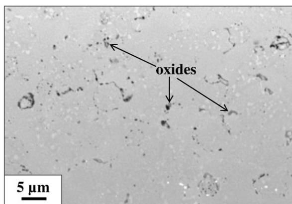
Fig. 11. Oxides within the \gamma\text{-Ni} matrix, in the inner part of the “Tribomet” Pt-modified NiCoCrAlYTa coating. SEM image in BSE mode.
