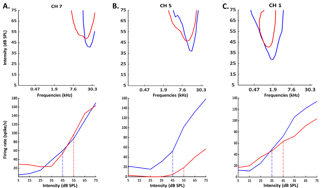
Figure 5. Examples of Frequency Response Areas (FRA) and rate-level functions (dB) obtained before and after CI insertion. Top: For each example, the blue curve represents the FRA obtained before CI insertion and the red curve the FRA obtained after CI insertion. Bottom: For each example, the blue curve represents the rate-level function obtained before CI insertion and the red curve the rate-level function obtained after CI insertion. A. In this case, the threshold (defined as a response above spontaneous activity plus 6 sem) increased from 45 to 55 dB and there was only a small decrease in evoked firing rate at 75 dB. B. In this case, the threshold (defined as a response above spontaneous activity plus 6 sem) increased from 45 to 55 dB and there was a large decrease in evoked firing rate at 75 dB. C. In this case, the threshold (defined as a response above spontaneous activity plus 6 sem) increased from 35 to 45 dB and there was a decrease in evoked firing rate at 75 dB. Note that in the three cases, there was not increase in the slope of the rate level function after CI insertion: the slope was either similar or slightly smoother after than before CI insertion.
