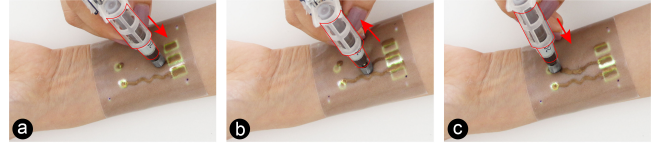
Figure 7: Constraints prevent invalid connections of conductive traces. The user draws a conductive trace to connect two terminals (a). As she is about to connect to another conductive trace and create a short-circuit, the pen retracts to non-inking mode (b). Moving the pen away from the original trace switches the pen back to inking mode (c).
