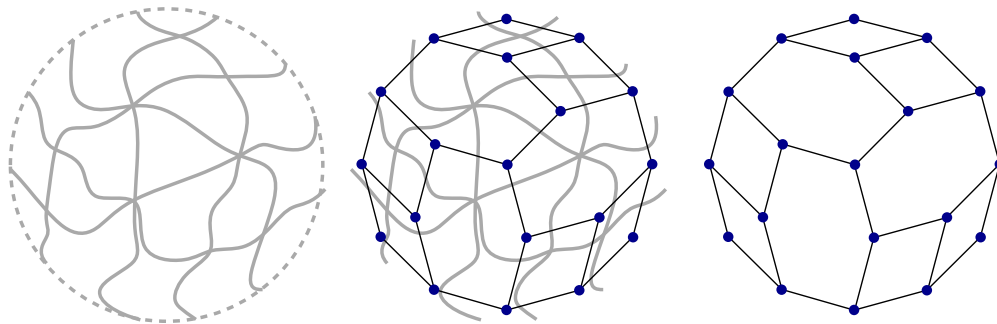
FIGURE 2. A pseudoline arrangement U and its region graph.
