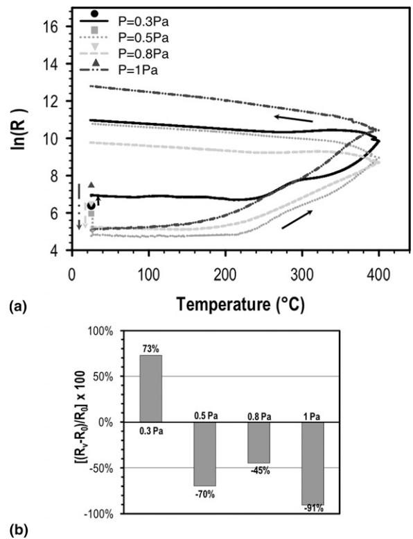
FIG. 4. Resistivity versus temperature measurements performed first in vacuum, and then in air for four samples deposited at 0.3, 0.5, 0.8, and 1 Pa. The stand-alone points mark the as-deposited resistivity for each sample, and the arrows indicate the direction of change in resistivity after the first vacuum annealing, thereby arriving at the “reference starting point” of each sample. Subsequent annealing and cooling in air results in a change of the resistivity as can be traced by the cyclic curves. In the inset, the percentage change in resistivity of each deposition pressure expressed as a function of the “reference starting point” is illustrated. R_0 is the as-deposited resistivity, while R_v is the resistivity after the first vacuum annealing. For the cycling curve at 0.5 Pa, the data points between 150 and 200 °C are deleted due to systematic disturbance to the signal as a result of noise during the electrical measurement. This region is marked with a solid line for visual guide.
