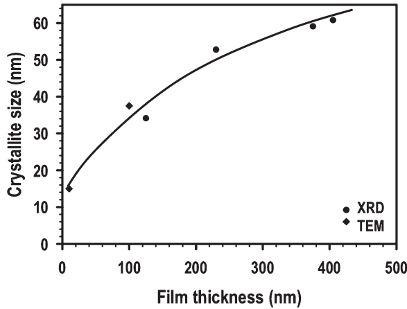
FIG. 3. Crystallite size as a function of the film thickness deposited at a constant pressure of 0.8 Pa.
