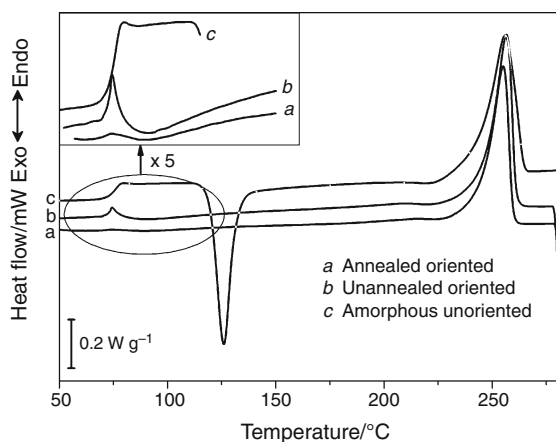
Fig. 1 DSC thermograms obtained with a heating rate of 10 °C \text{min}^{-1} on PET films. a Annealed oriented, b unannealed oriented, and c amorphous unoriented
