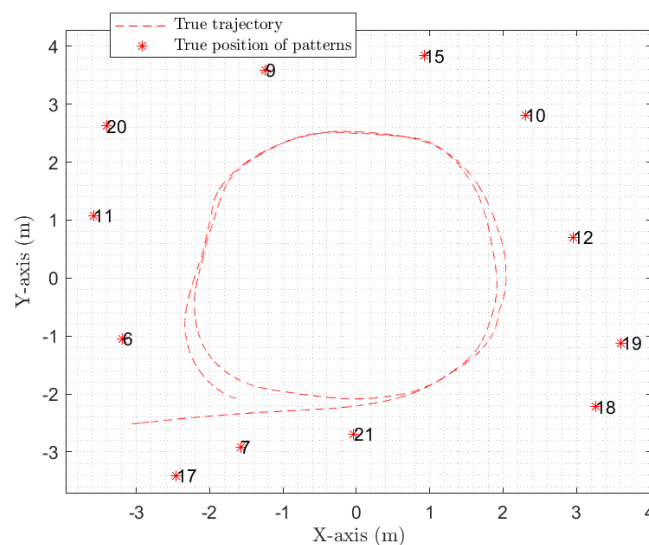
Figure 8. Ground truth obtained by an Optitrack motion capture system in the XY-plane, superimposed to the position of the center of the bottom-left ellipse of each coded pattern.
