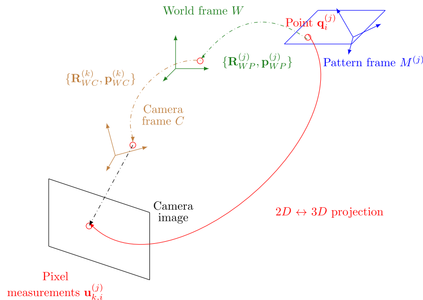
Figure 2. Geometrical representation of the projection camera model.
