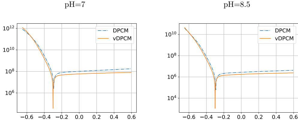
FIGURE 1. Evolution of the total current for the steady state (in physical units A \cdot m^{-2} ) in terms of the applied potential (in Volts) at pH = 7 and pH = 8.5
