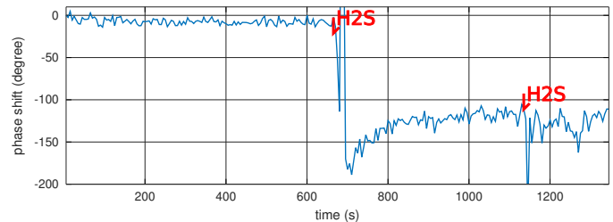
Fig. 8. Hydrogen sulfide ( \text{H}_2\text{S} ) detection by a functionalized SAW reflective delay line buried 30 cm deep in a sandbox. Hydrogen sulfide is produced and flow through the buried tube in which the sensor is located at time 700 s and 1150 s.
