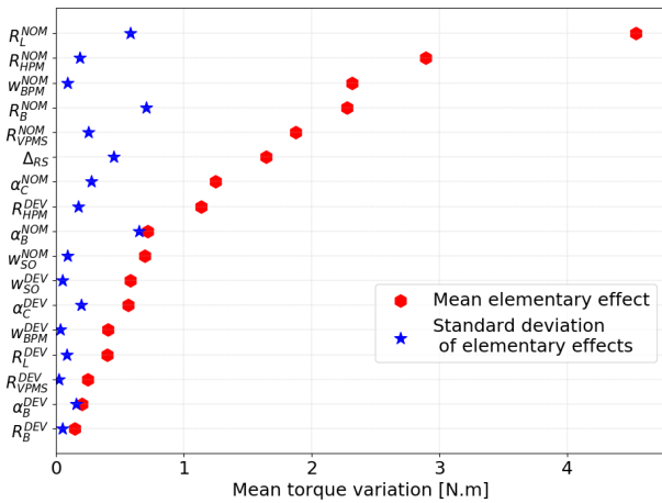
Fig. 4. Mean torque sensitivity to parameter variations.
