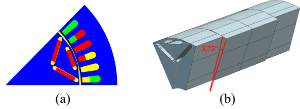
Fig. 1. Motor geometry.
