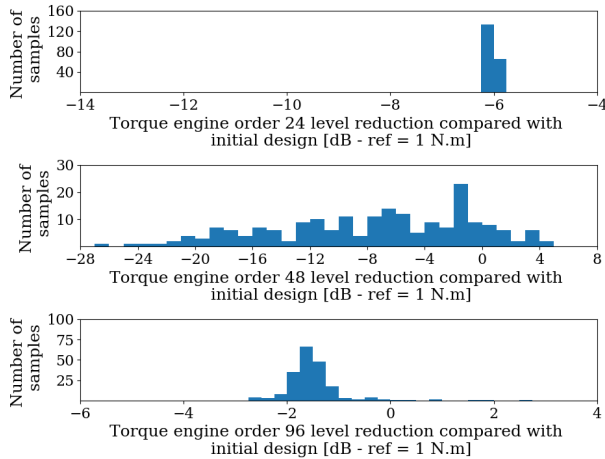
Fig. 13. Distribution of the objectives when considering deviations of the parameters \alpha_C , \alpha_B and R_{HPM}
