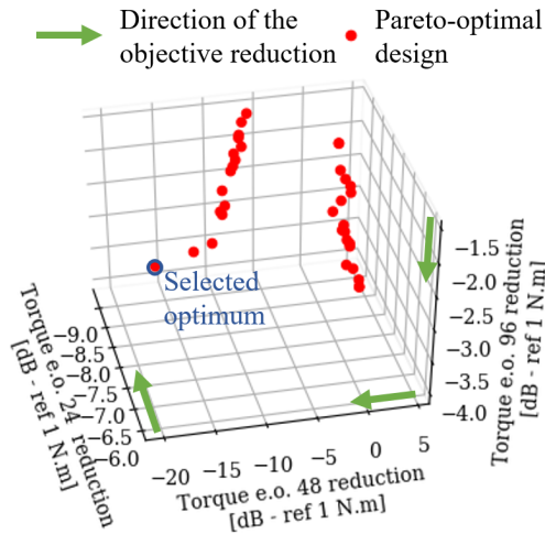
Fig. 10. Values of the objectives of the designs belonging to the estimated Pareto front for the classical multiobjective optimization aiming at minimizing the torque engine orders 24, 48 and 96 – first overview
