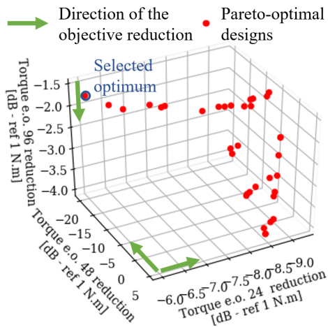
Fig. 11. Values of the objectives of the designs belonging to the estimated Pareto front for the classical multiobjective optimization aiming at minimizing the torque engine orders 24, 48 and 96 – second overview
