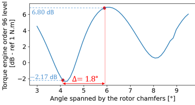
Fig. 9. Effect of the parameter \alpha_c on the torque engine order 96 level, for the design used to calculate its largest elementary effect due to deviations.
