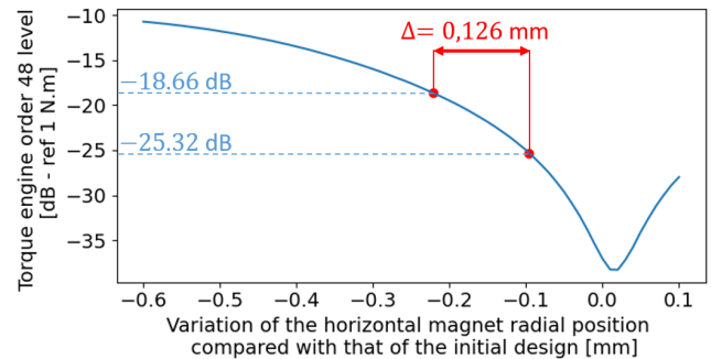
Fig. 8. Effect of the parameter R_{HPM} on the torque engine order 48 level, for the design used to calculate its largest elementary effect due to deviations.
