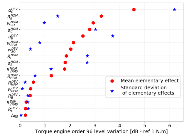
Fig. 7. Torque engine order 96 sensitivity to parameter variations.
