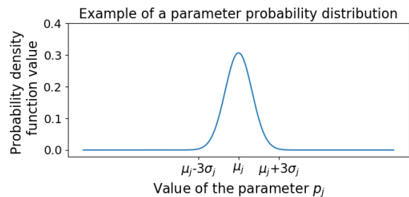
Fig. 12. Example of the normal probability density functions for a parameter p_j .
