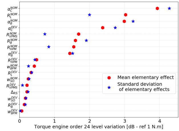
Fig. 5. Torque engine order 24 sensitivity to parameter variations.
