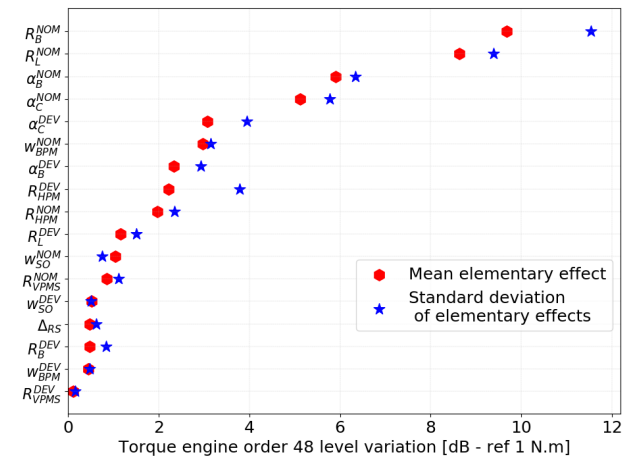
Fig. 6. Torque engine order 48 sensitivity to parameter variations.
