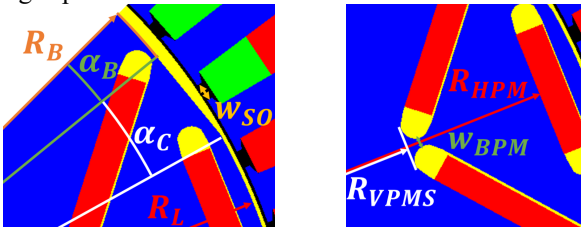
Fig. 3. Geometric parameters of the PMSM.
