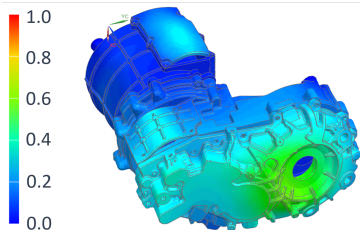
Fig. 2. Representation of the powertrain overall bending mode shape (1026 Hz) with unit maximum amplitude color scale.
