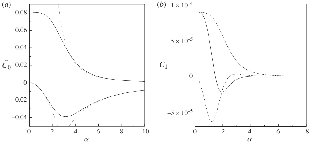
FIGURE 13. Hydraulic conductances for lubrication leading order in (a) and quadratic inertial corrections in (b). (a) The gap variations represented in figure 4(a,c) were chosen. \Re\{\tilde{C}_0\} is the upper continuous curve and \Im\{\tilde{C}_0\} is the lower continuous one. Dotted lines show the asymptotic behaviour of the homogeneous case (5.8). (b) The gap variations represented in figure 4(b,d) were chosen with \mathcal{D}/\mathcal{N} boundary conditions (4.2). \Re\{C_{1u}\} is the continuous curve and \Im\{C_{1u}\} is the lower dash-dotted line. The steady-streaming contribution C_{1s} is also represented by a dashed line.
