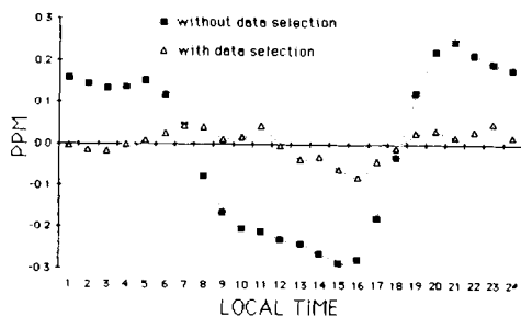
Fig. 2. Mean diurnal CO 2 variations for data without selection (squares) and for data corresponding only to the marine sector defined in the text (triangles).
