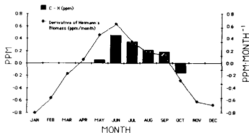
Fig. 7. The seasonal continental biomass component. \text{CO}_2 seasonal variation difference (bar) between air masses originating recently from South Africa (C) and the other air masses (X). Time derivative (black curve) of that part of Heimann's \text{CO}_2 seasonal variations due to the only continental biomass.
