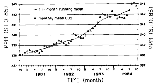
Fig. 3. Monthly mean CO 2 concentration after data selection (triangles) and 11-month running mean (black curve) at Amsterdam Island.
