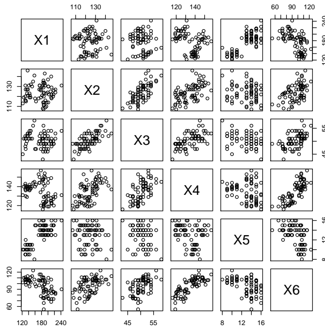
Figure 6: Scatterplot matrix of the Lubishew data.
