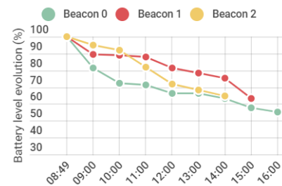
Figure 3: Battery level evolution
