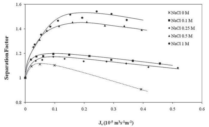
Fig. 8. Separation factor of NaLac purification from glucose vs. permeation flux for ternary solutions of glucose (0.1 M), NaLac (0.1 M) and NaCl: influence of the NaCl concentration.
