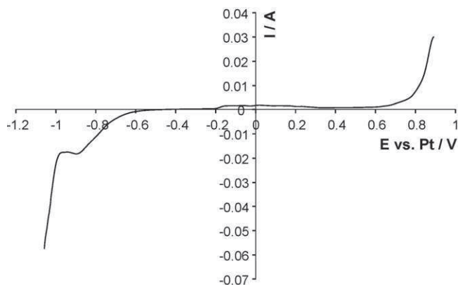
Fig. 14. Linear sweep voltammometry of LiF-CaF 2 -Th(IV) ( 6.77 \times 10^{-2} \text{ mol kg}^{-1} ) on liquid Bi electrode at 5 \text{ mV s}^{-1} and 840^\circ\text{C} . Auxiliary el.: vitreous carbon; comparison el.: Pt.
