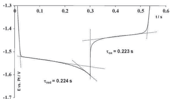
Fig. 5. Reversal chronopotentiogram of \text{ThF}_4 ( 0.101 \text{ mol kg}^{-1} ) in \text{LiF-CaF}_2 eutectic, i = -0.11 \text{ A} . Working el.: \text{Mo} ( S = 0.30 \text{ cm}^2 ); auxiliary el.: vitreous carbon; comparison el.: \text{Pt} .
