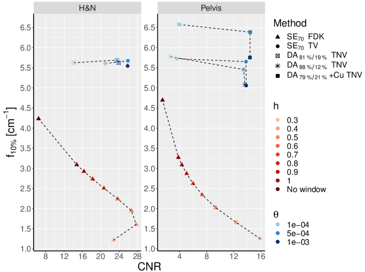
Figure 1 CNR and spatial frequency for the best scans of FDK, SE TV, and DE (DA) TNV (LE component, N=10) for the H&N (left) and pelvis (right) phantom configuration. For the pelvis (right) phantom configuration, an example with additional beam filtration is displayed as well.
