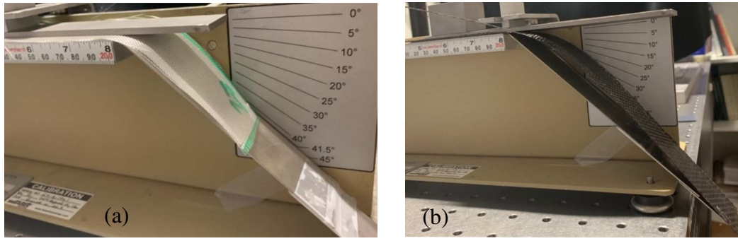
Fig. 5. Cantilever bending test. (a) Glass plain weave. (b) Carbon 5 harness satin weave.
