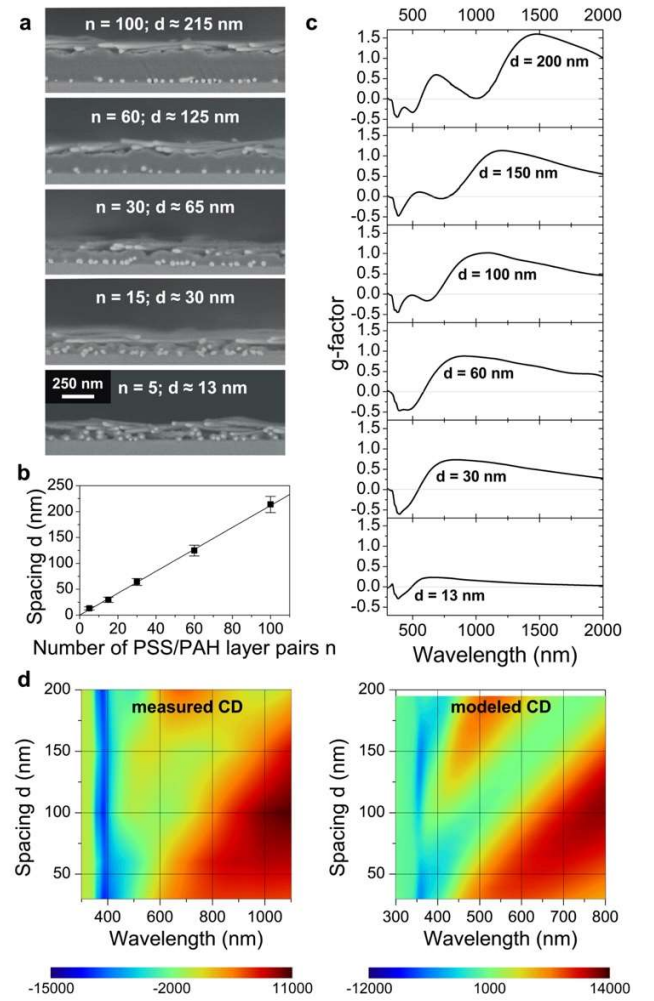
Figure 3. Variation of the spacing d between the AgNW layers. a) Cross-section SEM images of two-layer structures with varying interlayer spacing d . b) Interlayer spacing d as a function of number of PSS/PAH layer pairs n . c) g-factor spectra of two-layer structures with increasing interlayer spacing d . d) Measured (left) and modeled (right) CD spectra as function of the interlayer spacing d (note the different wavelength scale and the different color scale coding for the CD in mdeg).
