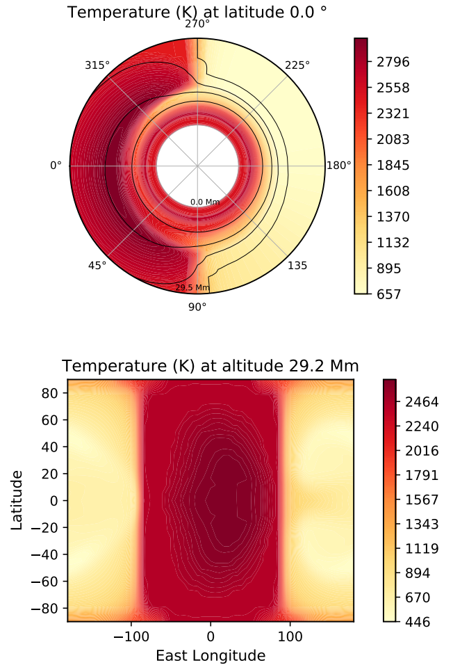
Fig. 9. Temperature maps of WASP-121b. The top map shows an equatorial slice. The planet radius is divided by 10 for visual reasons. The black lines correspond to different isobar levels. The bottom map shows a slice at high altitude (29.2 Mm, i.e., 29 200 km). The hottest point is slightly shifted to the east limb, i.e., the trailing limb.
