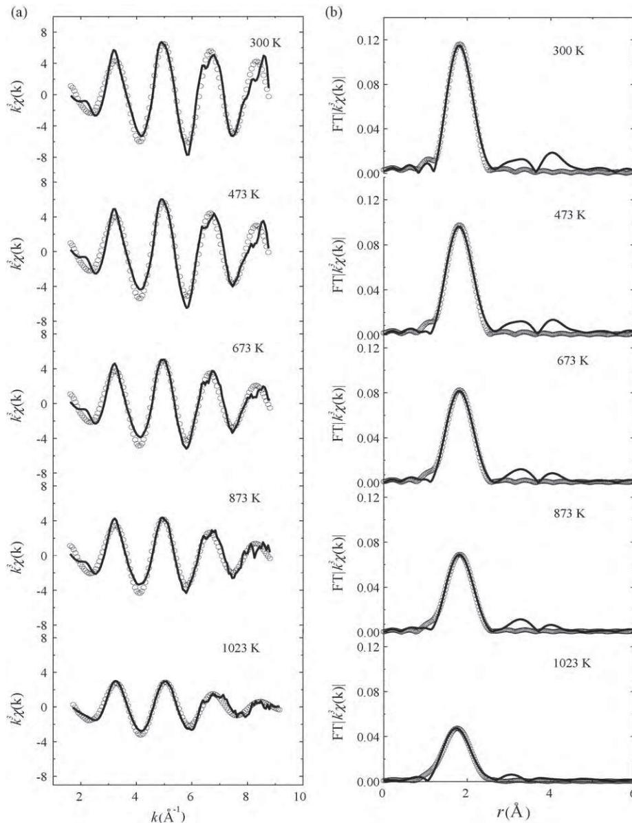
Fig. 1. (a) and (b) Tb L_{\text{III}} -edge XAFS oscillations, k^3\chi(k) , and radial structural functions, \text{FT}|k^3\chi(k)| , of 20Tb–80Li at various equilibrated temperatures.
