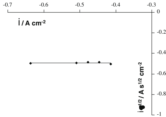
Fig. 6. Linear relationship between i\tau^{1/2} and the applied current density. T = 840 \text{ °C} and C = 2.97 \times 10^{-4} \text{ mol cm}^{-3} . Working EL: Mo ( S = 0.392 \text{ cm}^2 ); auxiliary EL: vitreous carbon; quasi-reference EL: Pt.
