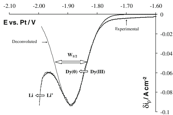
Fig. 7. Typical square wave voltammogram of the LiF–CaF 2 –DyF 3 ( 9.4 \times 10^{-5} \text{ mol cm}^{-3} ) system at frequency f = 9 \text{ Hz} and T = 840 \text{ °C} . Working EL: Mo ( S = 0.314 \text{ cm}^2 ); auxiliary EL: vitreous carbon; quasi-reference EL: Pt.
