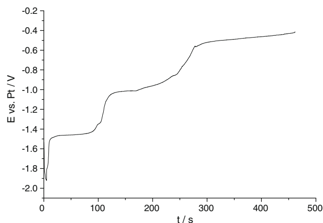
Fig. 10b. Open-circuit chronopotentiograms of LiF-CaF 2 -DyF 3 ( 9.4 \times 10^{-5} mol cm -3 ) system on copper electrode at T = 840 °C. Auxiliary EL.: vitreous carbon; quasi-reference EL.: Pt.
