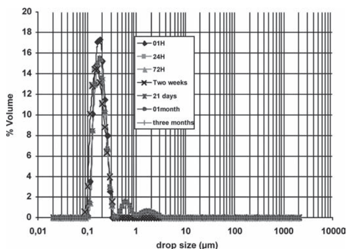
FIG. 26. Volume percentage of droplet size distribution of T22/ C_{12}E_4 emulsion versus drop size at optimal conditions (1 wt% surfactant, 60 s, 7500 rpm) (kinetic stability performed with Ultrazizer measurements).
