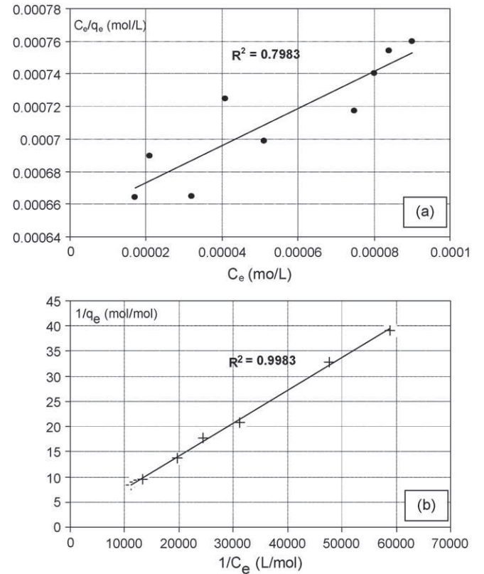
Fig. 5. Characteristic linear plots of Langmuir isotherm for \text{pH}_i 7, [\text{F}^-]_0 = 15 \text{ mg/L} , \kappa = 7.5 \text{ mS/cm} , j = 17.1 \text{ mA/cm}^2 : (a) C_e/q_e vs. C_e (Eq. (2)); (b) 1/q_e vs. 1/C_e (Eq. (3)).
