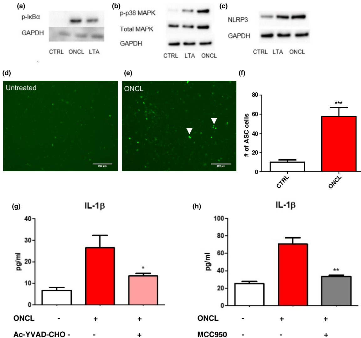
Figure 3 ONCL induced inflammation-signalling pathway. Representative images of western blots for (a) Phospho-IkB \alpha (b) phosphorylated p38 MAPK, total MAPK, and (c) NLRP3 at the predicted molecular size on THP-1 macrophages treated with ONCL. LTA was used as positive control. (d, e) representative images from live cells imaging of THP-1 ASC-FGP macrophages showing ASC formation following ONCL treatment. The number of ASC positive cells is higher in ONCL treated compared to untreated cells (f). To confirm inflammasome activation with ONCL, pretreatment with both caspase-1 inhibitor, Ac-YVAD-CHO and NLRP3 inhibitor MCC950 significantly reduced the levels of IL-1 \beta release (g, h). Data represent average of three independent experiments and presented as mean \pm SEM. * P < 0.01 , ** P < 0.001 , ANOVA with Bonferoni correction.
