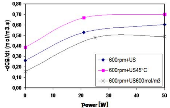
Fig. 7 Initial apparent reaction rate versus ultrasound power for different operating conditions
