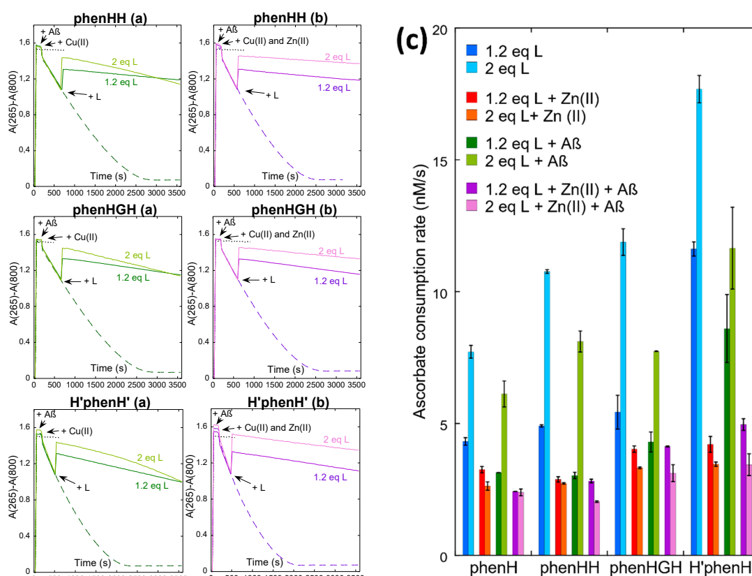
Figure 2. Kinetics of ascorbate consumption, starting from a mixture of Cu(II) and Cu(I), with Aβ, without (a) or with (b) Zn(II), without (dashed line) or with (plain line) 1.2 or 2 equivalents of L (ligand), followed by UV-vis spectroscopy at 265 nm with a background correction at 800 nm. [\text{AscH}^-] = 100 \mu\text{M} , [\text{Cu}] = 10 \mu\text{M} , [\text{A}\beta] = [\text{Zn}] = 12 \mu\text{M} , [\text{L}] = 12 or 20 \mu\text{M} , [\text{HEPES}] = 100 \text{ mM} , pH 7.1. Black dotted lines indicate the control experiment with ascorbate only. (c) Ascorbate consumption rate, between 2000 and 3000 s, calculated by dividing the slope of the variation of absorbance by the extinction coefficient of ascorbate, \epsilon_{265 \text{ nm}} = 14,500 \text{ M}^{-1} \text{ cm}^{-1} . Data are means \pm S.D. Measurements were performed on at least two independent experiments ( n = 2/3 ).
