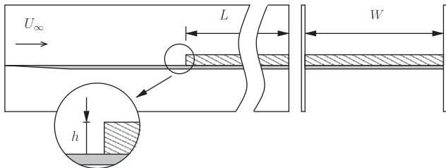
Fig. 2. Schematic of the polycarbonate and acrylic experimental model used in the current study. Height of end is 210 mm.
