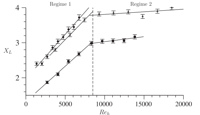
Fig. 8. Variation of X_L with Re_h for three \delta/h ratios, 0.83 < \delta/h < 2.5 : \bullet : \delta/h = 2.5 ; \blacksquare : \delta/h = 1.25 ; and \blacktriangle : \delta/h = 0.83 .
