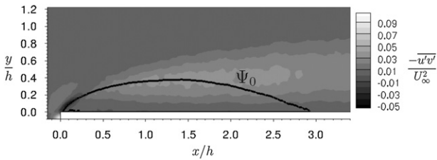
Fig. 7. Reynolds shear stress contours produced above a FFS for \delta/h = 1.25 ; Re_h = 6741 , contours of -\bar{u}'\bar{v}'/U_\infty^2 ; solid line is the dividing streamline \Psi_0 .
