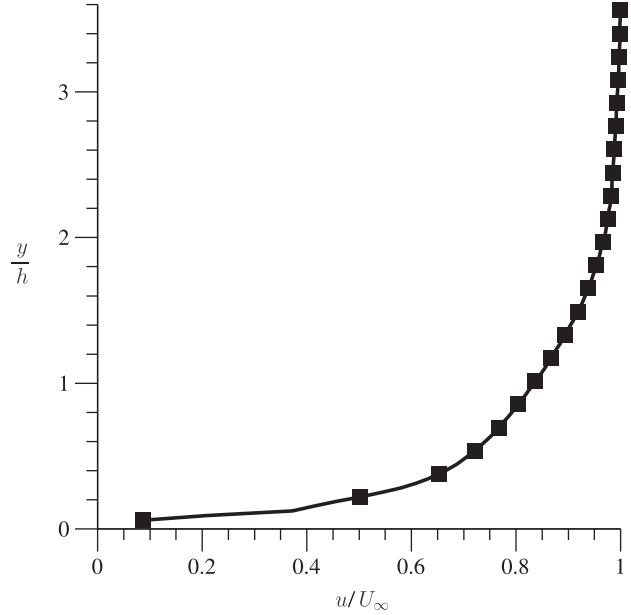
Fig. 3. The upstream boundary layer profile measured at 9h_{h=15 \text{ mm}} upstream of the step using 2500 independent PIV images. Only every fifth data point is presented for clarity.
