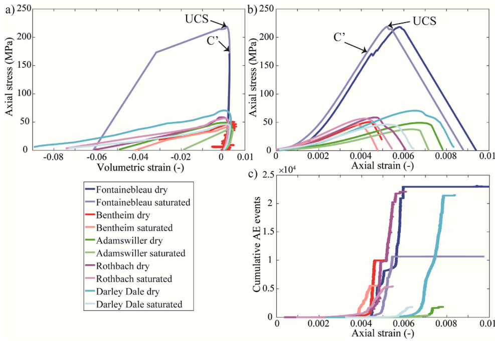
Fig. 4. Mechanical and AE data obtained for the uniaxial compression tests of the five sandstones deformed under dry and water-saturated conditions. a) Axial stress as a function of the volumetric strain, b) axial stress as a function of the axial strain and c) cumulative AE events as a function of the axial strain. An example of C' and the UCS is shown for a Fontainebleau sandstone experiment performed under water-saturated conditions. Note that the AE data are very well correlated with the mechanical data, presenting an increase in events before and at each stress drop.
